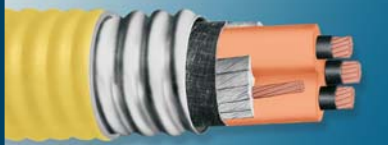
2.4 kV CLX Non-Shielded (UL) MV-90, Type CT, MC-HL, EP-PVC
